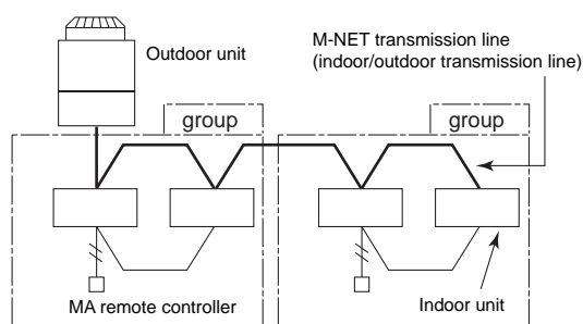
<System with MA remote controller>
